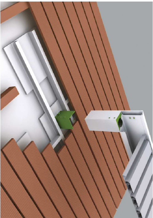
fixing on the terrace without anchoring
